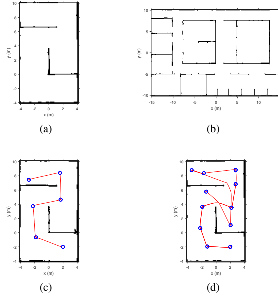
Fig. 3: (a) Curving hallway environment used with 1 robot; (b) larger office environment used with 5 robots; and simulation results for the curved hallway for frontier (c) and angle aware (d) planning methods. The red line shows the path of the robot and the blue circles represents panorama capture locations.
