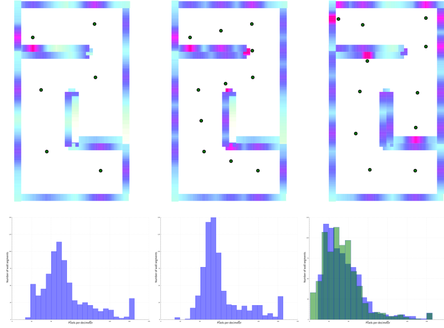
Fig. 4: Top row: map renderings with walls colorized by the resolution at which they were covered for frontier (left), augmented frontier (center), and angle aware (right) approaches. Hue indicates imaging resolution with red indicating high resolution, and blue indicating low resolution. In grayscale, the less saturated wall segments indicate poor coverage. Panorama capture locations are denoted by green circles. Bottom row: histograms of pixels per decimeter for augmented frontier (left), angle aware (center), and augmented frontier overlaid on angle aware (right).
