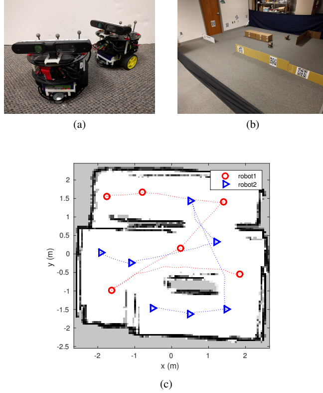
Fig. 6: The ground robots (a), lab space used for live experiments (b), and experimental results showing the panorama capture locations for the two robot team (c).
