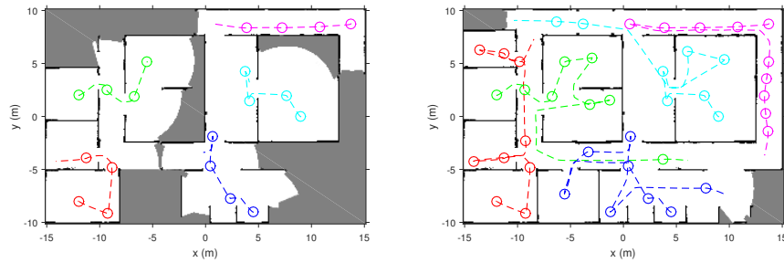
Fig. 5: Five robots collaboratively exploring an office environment after 4 panoramas (left) and after 10 panoramas (right).
