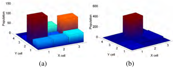
Fig. 13. Population distribution for a swarm of 500 mobile sensors over a period of 60 sec (a) with no controls, i.e. , passive, and (b) with controls with T_c = 0.8T_a .
