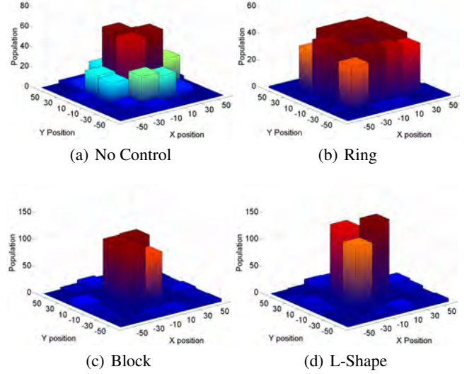
Fig. 5. Histogram of the final allocations in the time-invariant flow field for the swarm of (a) passive robots exerting no controls and robots exerting control forming the (b) Ring pattern with T_c = 0.8T_a at t = 450 , (c) Block pattern with T_c = T_a at t = 450 , and (d) L-shape pattern with T_c = 0.5T_a at t = 450 .
