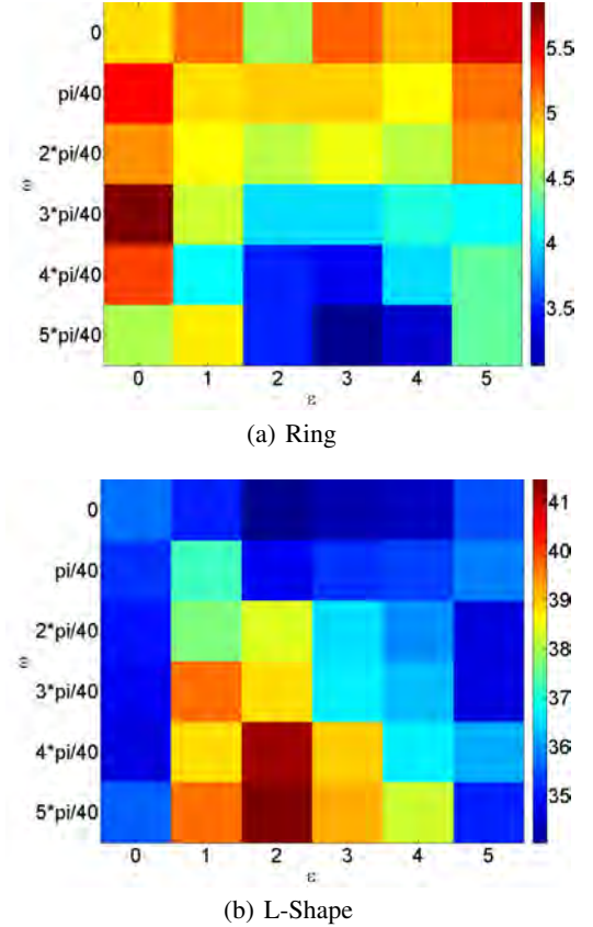
Fig. 9. Final population RMSE for different values of \omega and \varepsilon for (a) the Ring formation and (b) the L-shaped formation.
